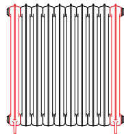
920 x 852 10 sections (2+8)
