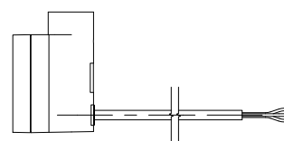
Straight cable without plug; Fil Pilote connection
